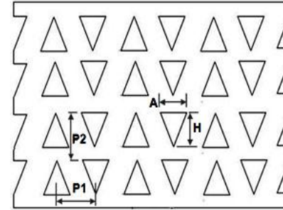
Triangle Hole Staggered Pattern
