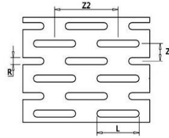
Slot Hole Round End "Z" Staggered Pattern
