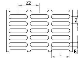
Slot Hole Round End 90° Straight Pattern
