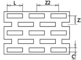
Slot Hole "Z" Staggered Pattern
