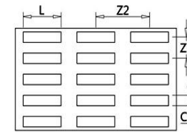
Slot Hole 90° Straight Pattern
