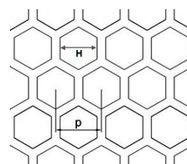
Hexagonal Hole
