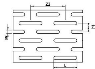
Z Type Slotted Hole
