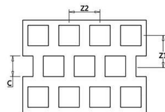
Z Type Square Hole
