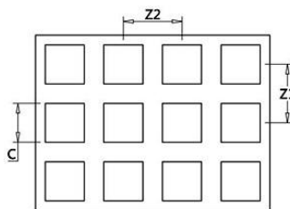
90° Square Hole
