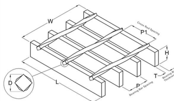
Pressure Welded Grating
