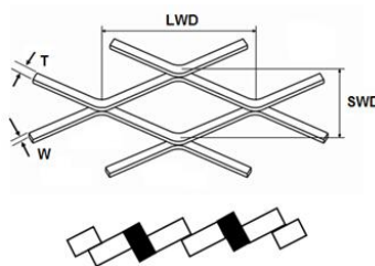
Standard Type Expanded Metal
