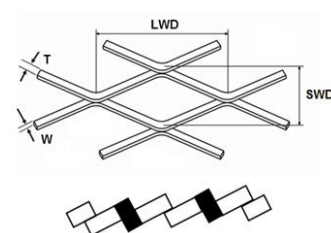
Diamond Hole Expanded
