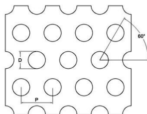
Round Hole Perforated
