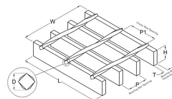
Press-locked Steel Grating
