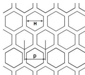
Hexagonal Hole
