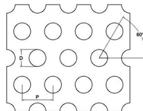
60° Round Hole Perforated
