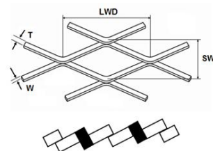
Hexagonal Hole Expanded
